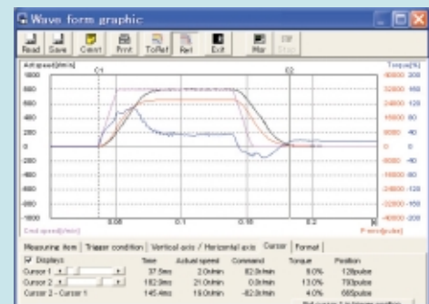
Graphic waveform display
